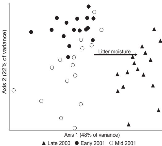
Fig. 4. Nonmetric Multidimensional Scaling (NMS) plot of the litter arthropods according to the growing seasons (Late 2000, Early 2001, and Mid 2001) in 48 litter samples from the thinning treatments. Growing seasons represented the sampling times during 2000 and 2001. (Moisture correlated with axis 1 at 78% and axis 2 at 48%; minimized final stress = 19.09%; Final instability = 0.00001; Monte Carlo 50 runs).
