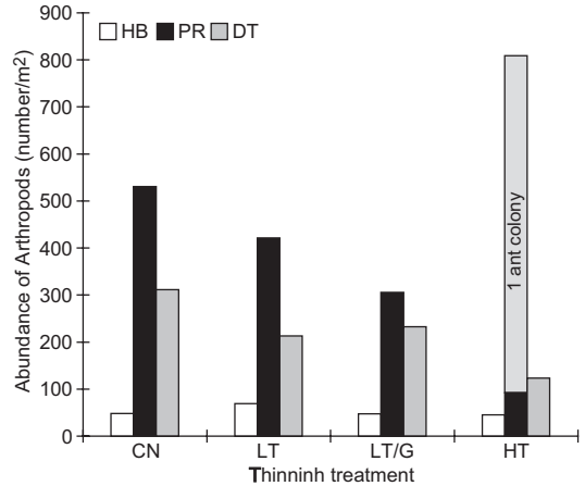
Fig. 2. Total abundance (excluding Collembola and mites) of functional groups of litter arthropods at each thinning treatment. HB = herbivores, PR = predators, DT = detritivores. As in Fig. 1, the effect of the inclusion of a single ant colony is specifically noted because it affects the interpretation significantly; the ants in this sample (one species) were excluded from analyses.
