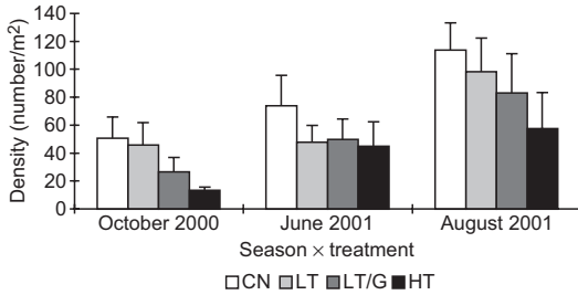
Fig. 1. Mean density of litter-dwelling arthropods in the different growing seasons and thinning treatments. CN = Control; LT = Light Thin; LT/G = Light with Gap; HT = Heavy Thin. Late 2000, Early 2001, Mid 2001.
