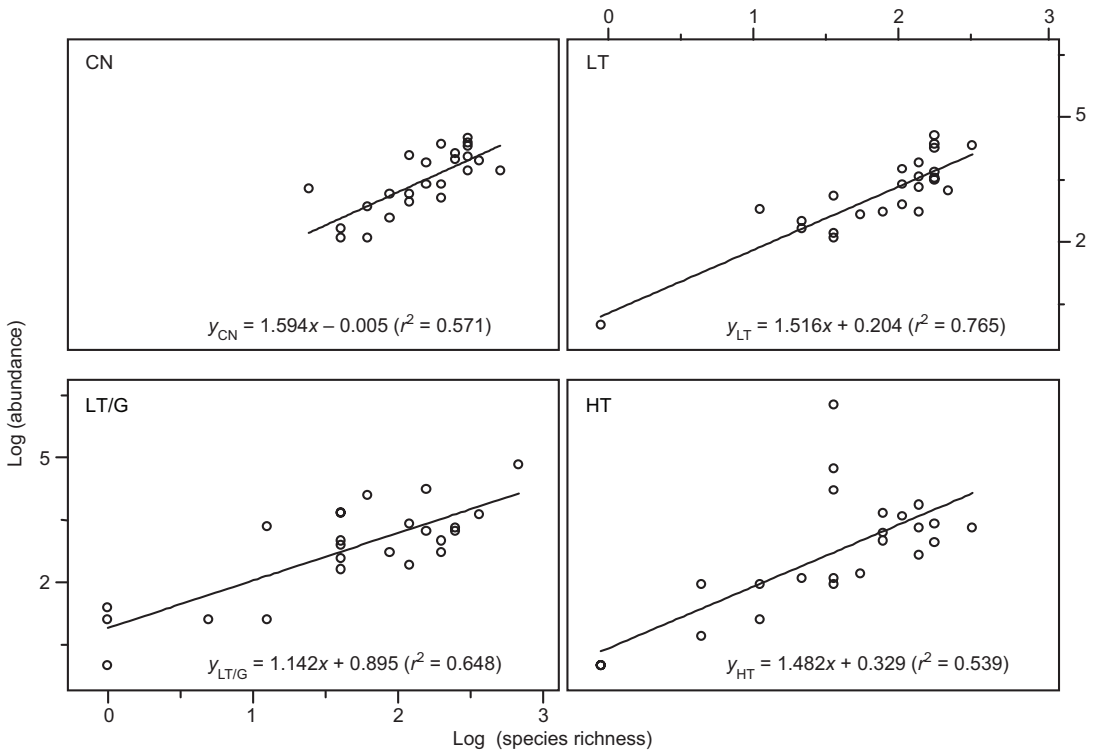
Fig. 3. Regression of log species richness versus log total abundance for the four thinning treatments.
